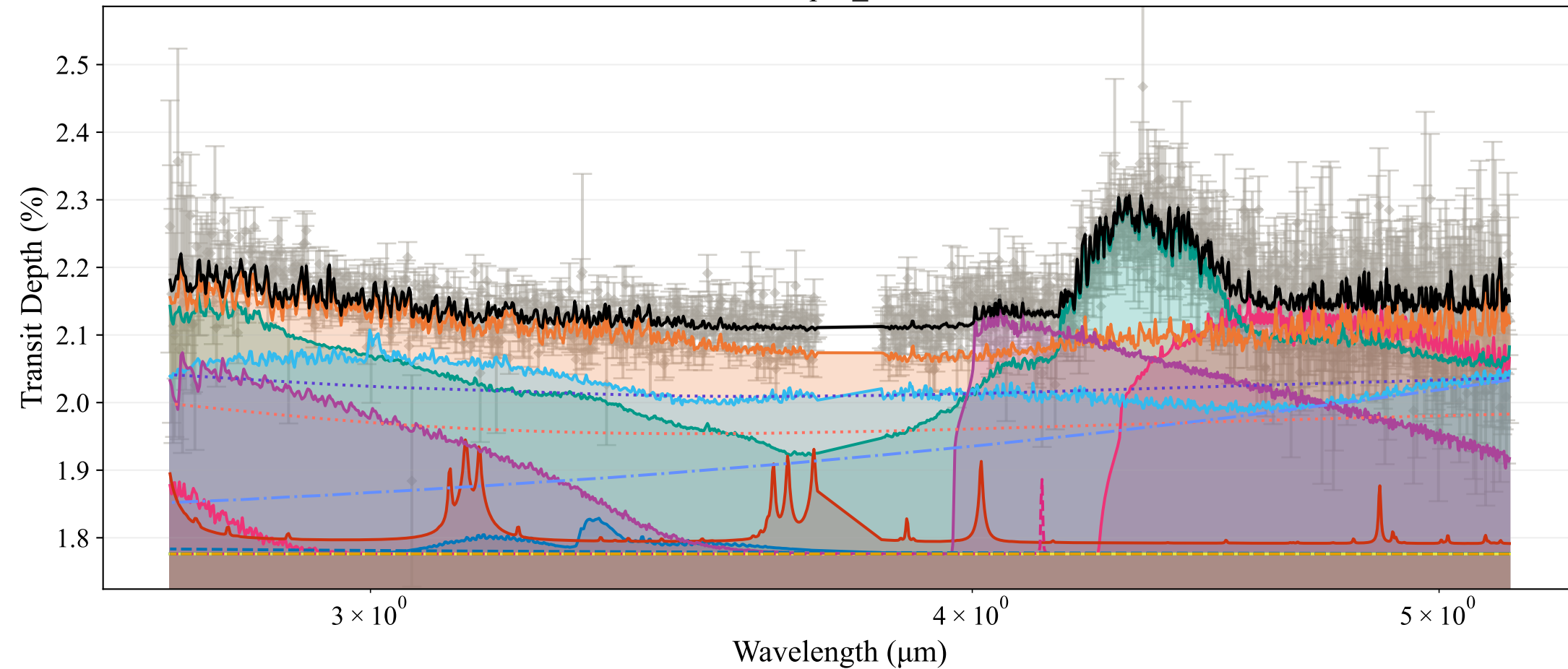
nirspec_SiO
